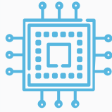
Automation Testing
