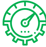
Stress & Performance
